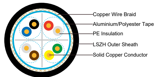
SF/UTP CAT6
